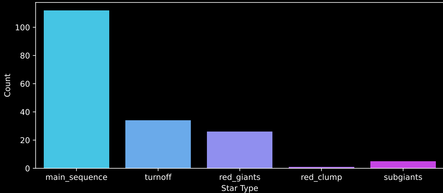
APOGEE DR17 Field: [350+87_MGA] Count plot of Star Type
