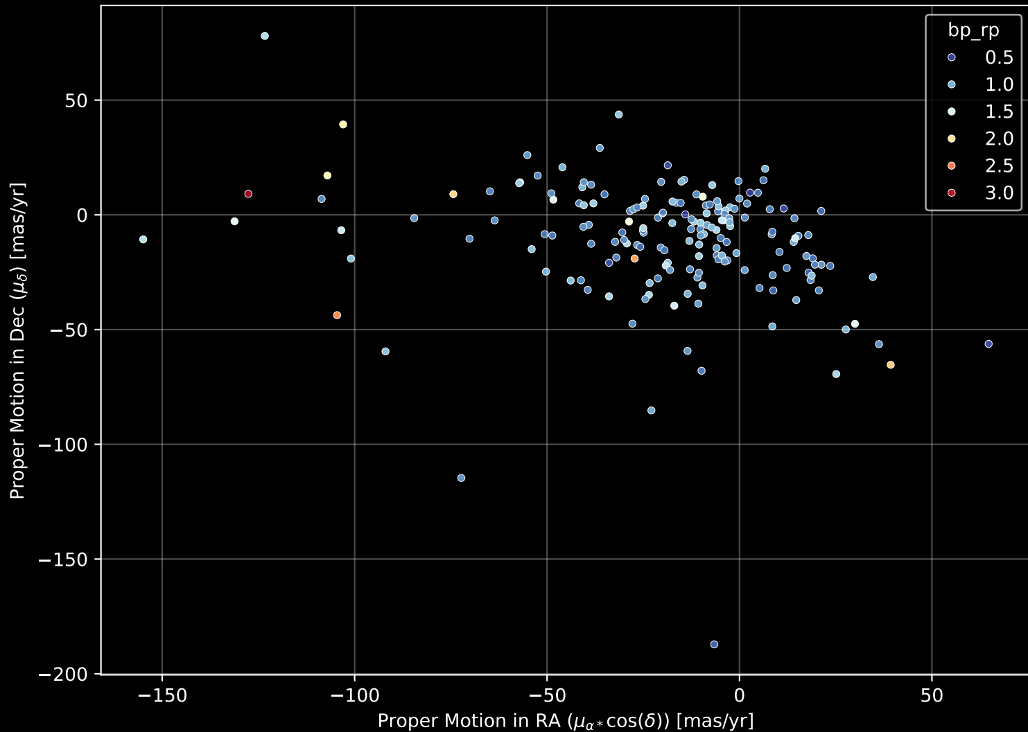
APOGEE DR17 Field: [350+87_MGA] Proper Motion Diagram (n= 178)
