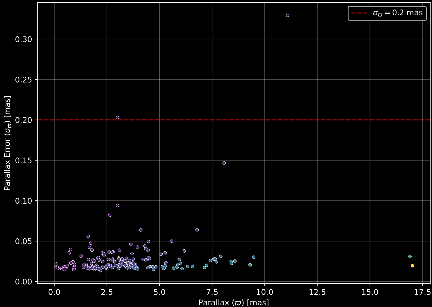
APOGEE DR17 Field: [350+87_MGA] Parallax Quality (n= 178)
