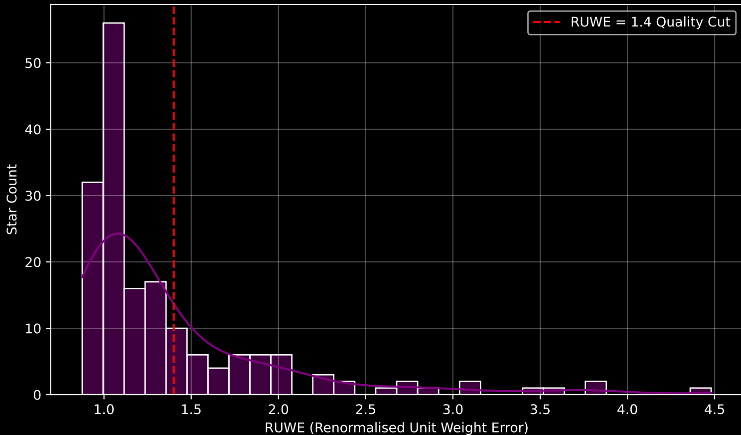
GAPOGEE DR17 Field [350+87_MGA] RUWE Distribution (n= 175)
