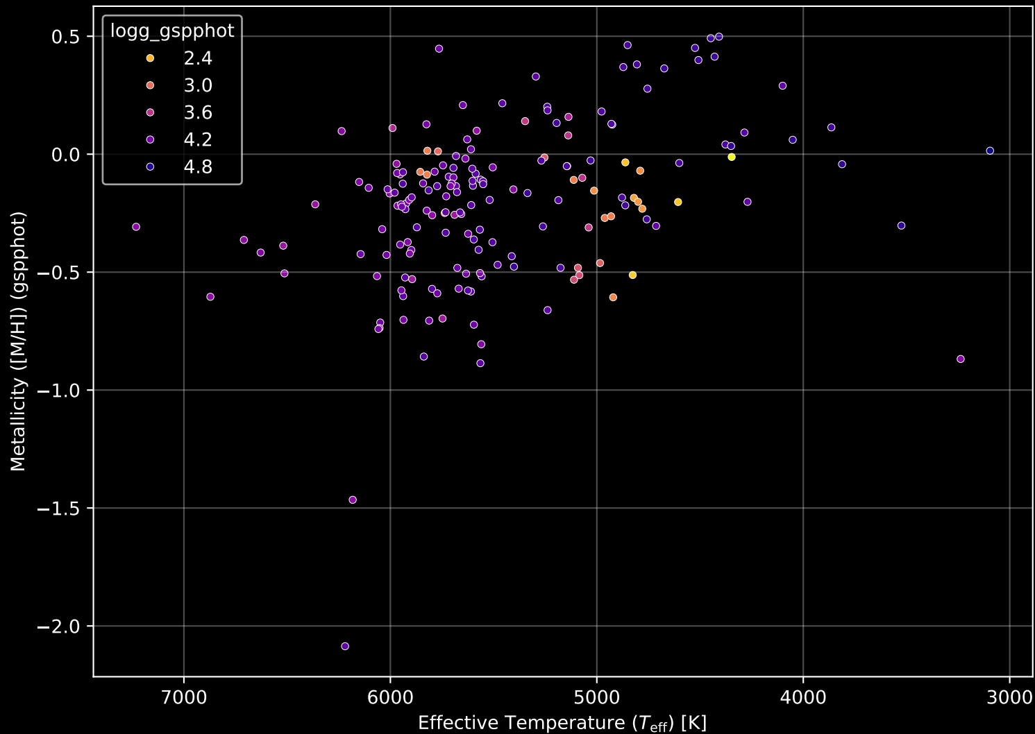
APOGEE DR17 Field: [350+87_MGA] Stellar Population Parameters (n= 178)
